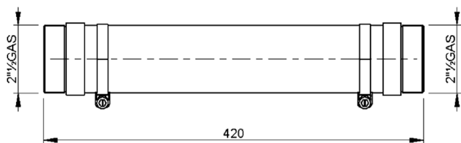
MANICOTTO FLESSIBILE FLEXIBLE HOSE tipo-type: FH8
