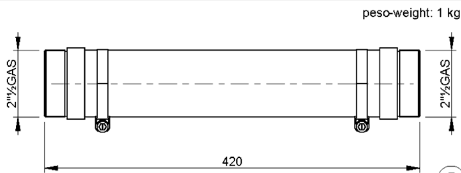
MANICOTTO FLESSIBILE FLEXIBLE HOSE tipo-type: FH8
