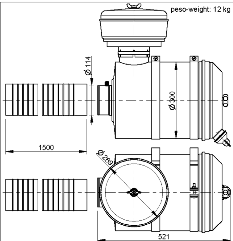
FILTRO BISTADIO DOUBLE STAGE FILTER per ambienti polverosi e desertici for dusty and sandy environments FDS 14/10
