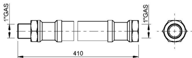
3 - FH4 MANICOTTO FLESSIBILE FLEXIBLE HOSE
